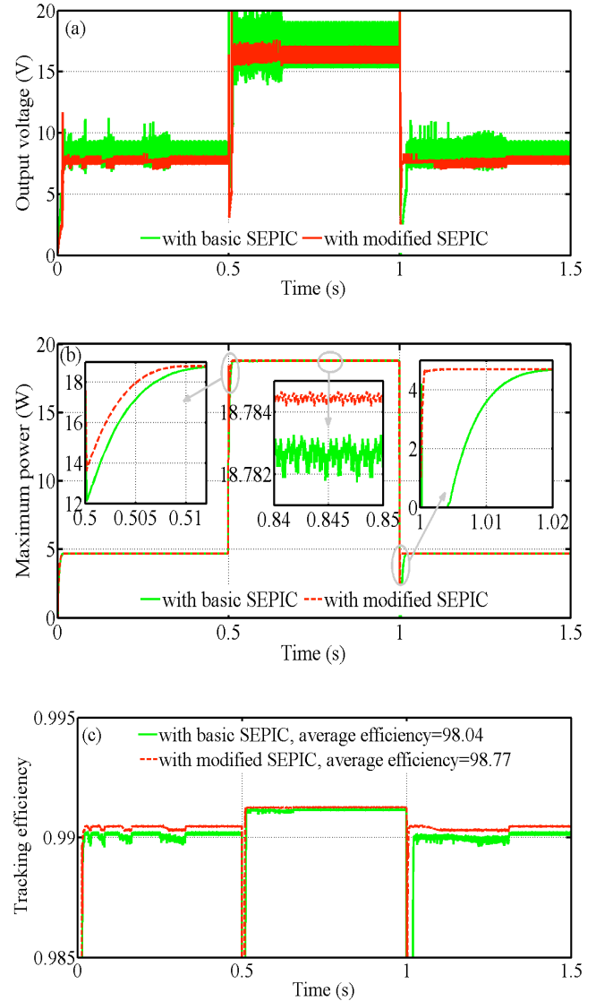
Fig. 8 – Comparison basic vs. Modified SEPIC: (a) Output voltage, (b) Maximum power, (c) Average efficiency.
