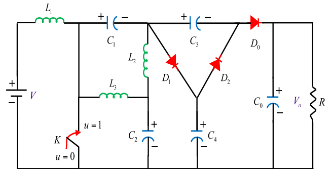
Fig. 3 – Modified SEPIC structure.
