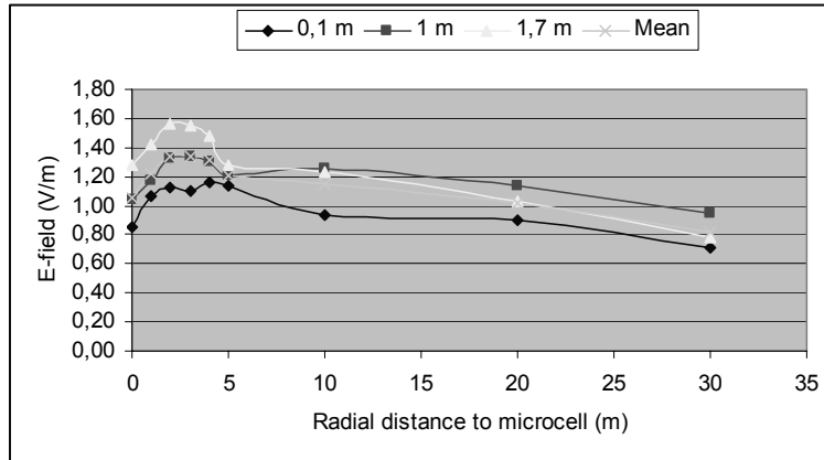
Fig. 8 – Relation between E -field strength, measurement height and radial distance to microcell.
