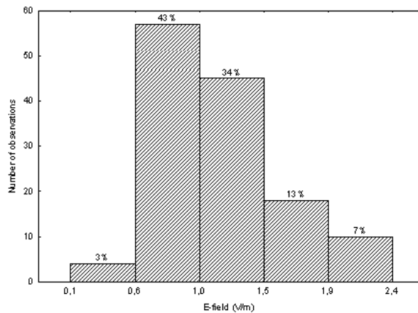
Fig. 7 – Histogram of the peak E -field.
