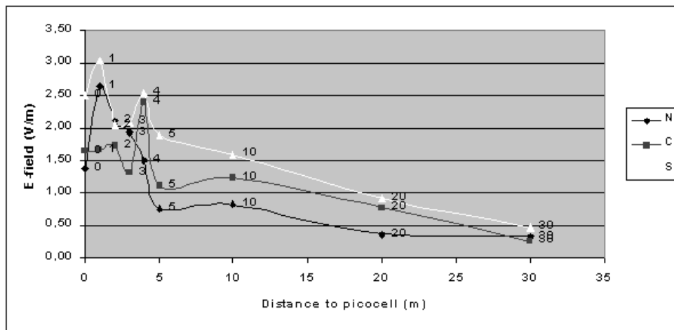
Fig. 5 – E -field versus distance in the Brussels railway stations North (N), Central (C) and South (S).
