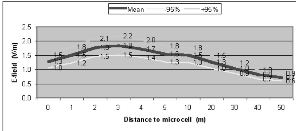
Fig. 11 – Average RF-exposure recorded in 30 randomly selected streets.
