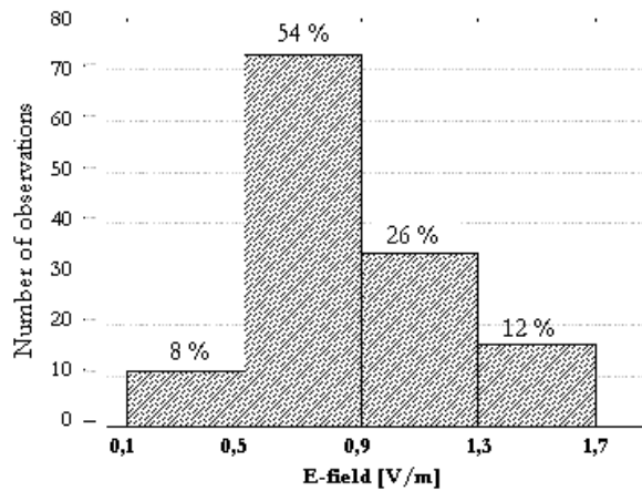
Fig. 6 – Histogram of RMS E -field.
