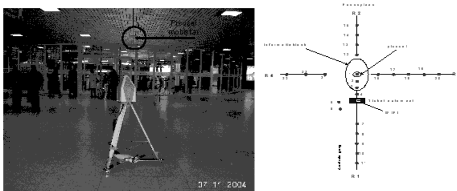
Fig. 1 – Setup example for evaluating the indoor E -field exposure of picocells.
