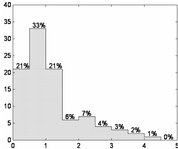
Fig. 10 – Distribution histogram of the RF-exposure in the shopping streets (worst case situation).
