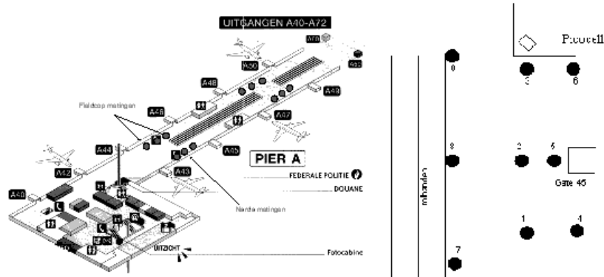
Fig. 3 – Measurement scheme in the PIER A for evaluating the E -field distribution in the waiting rooms at the different gates.
