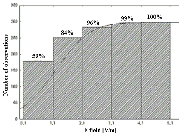
Fig. 9 – Cumulative distribution of the E -field strength in the shopping streets.
